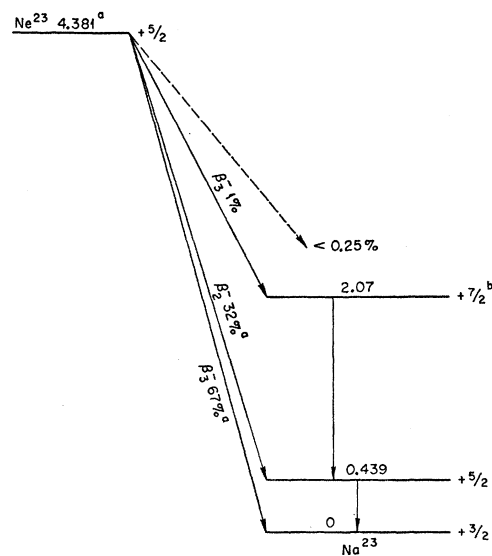
FIG. 2. Decay scheme for \text{Ne}^{23} . Energies are in units of MeV. Most of the data are taken from J. R. Penning and F. H. Schmidt, Phys. Rev. 105 , 647 (1957). See also (a) the present paper, (b) D. W. Braben, L. L. Green, and J. C. Willmott, Proceedings of the Rutherford Jubilee International Conference (Heywood and Company Ltd., London, 1961), p. 265.
