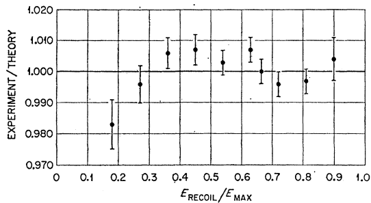
FIG. 3. Comparison of the experimentally determined recoil spectrum of (\text{Ne}^{23})^+ with theory, where \alpha = -0.329 , E_{\text{max}} = 553 eV, and the beta-ray intensities are those given in Fig. 2.
