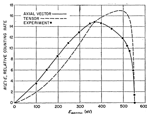
FIG. 1. Recoil spectrum of (\text{Na}^{23})^+ following the \beta^- decay of \text{Ne}^{23} . The experimental data are compared with special shapes as calculated for axial-vector and tensor interaction.
